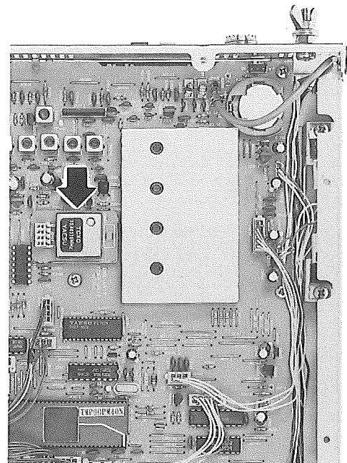
Figure 8: TCXO Installation
