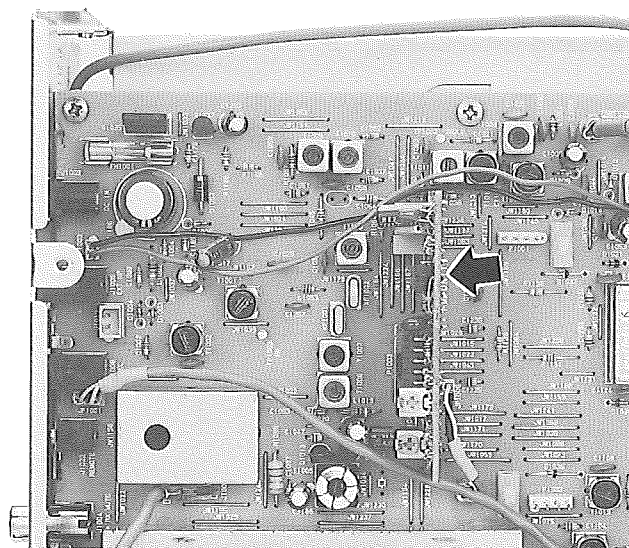
Figure 3: FM Unit Installation
