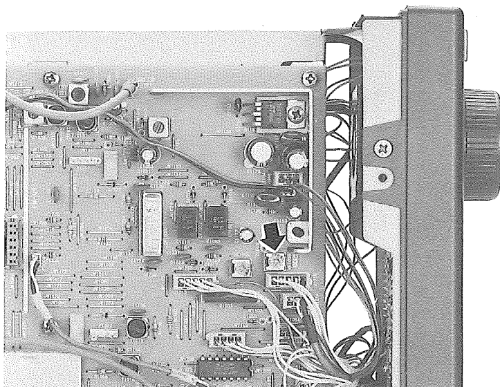
Figure 1: Top Cover Removal
